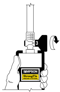
9. Turn the black valve to the #3 position and remove the black cap from the end of the nozzle. If performing gravity feed, the material is ready to dispense. If performing pressure injection, attach the E-Z-Click™ injection fitting to the end of the nozzle.
